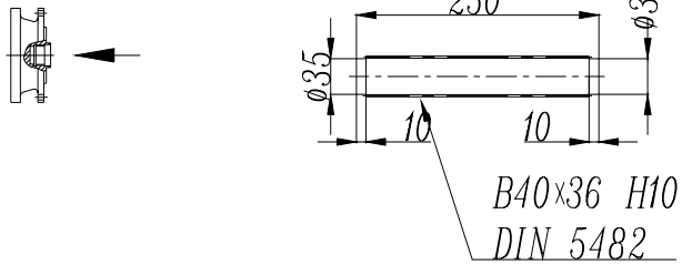
Splined bars
